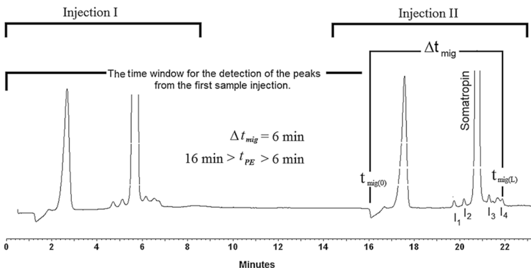
Fig. 3 Analysis of somatropin reference standard in single- (a) and double-CZE modes (b). Running conditions: a PB/CS double-coated capillary of dimensions 70 \times 60 \text{ cm} \times 50 \text{ }\mu\text{m} was used. Separation was performed at 17.4 kV (90 \mu\text{A} ) at 30 °C. Prior to the second injection, the first injected sample was electrophoresed at 17.4 kV for 15 min ( t_{\text{PE}} )
