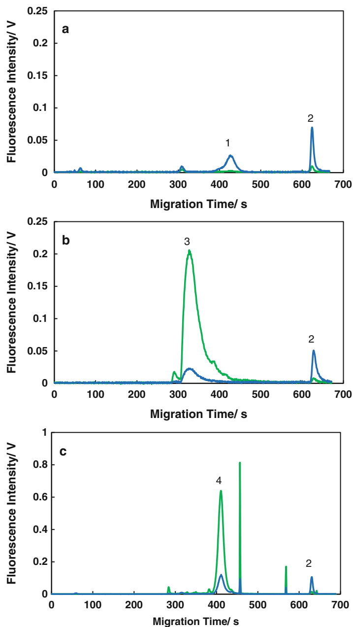
Fig. 5 Electropherograms of thyroglobulin, Rh-Con A, and their mixture. (a) 4.9 \mu M thyroglobulin (sample 1), (b) 4.9 \mu M Rh-Con A (sample 2), (c) a mixture of 4.9 \mu M thyroglobulin and 4.9 \mu M Rh-Con A (sample 3). (1) thyroglobulin, (2) fluorescein, (3) Rh-ConA, (4) complex between thyroglobulin and Rh-Con A. Blue lines and green lines are obtained by 450-nm excitation and 532-nm excitation, respectively. Reproduced from [15] with permission from John Wiley and Sons
