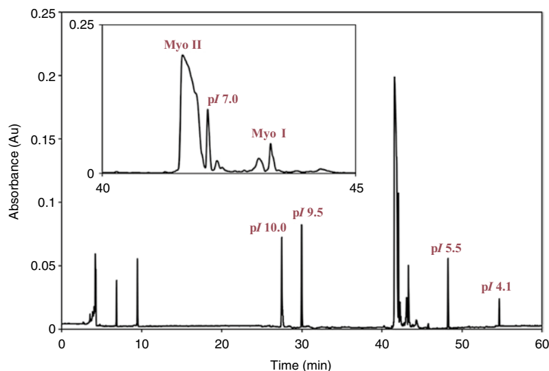
Fig. 3 A representative electropherogram of a complete cIEF experiment using p/3–10 carrier ampholytes and 5 peptide p/standards at p/ 10.0, 9.5, 7.0, 5.5, and 4.1. Two myoglobin isoforms were observed as labeled in the inset. Inset: magnified electropherogram from 40 to 45 min
