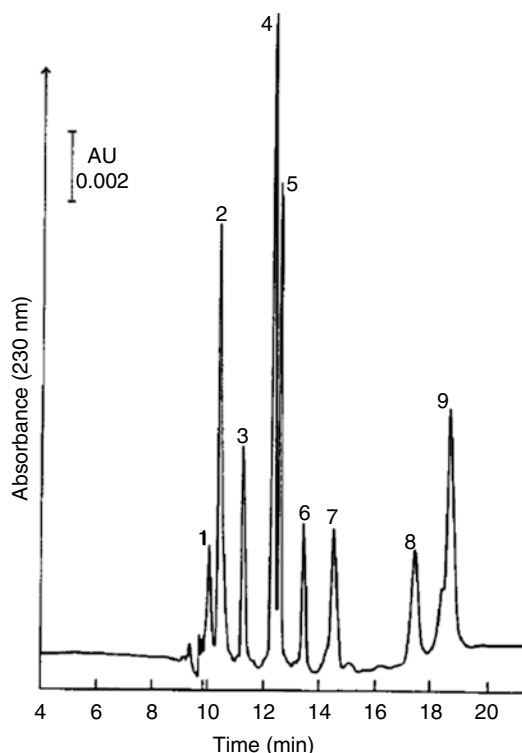
Fig. 2 Electropherogram of separated protein mixture in capillary filled with 6 % polyacrylamide. Total capillary length is 45 cm, with a length to the detector of 25 cm, and capillary id is 75 \mu m. Separation voltage is 12 kV, and running buffer is 0.1 M Tris-HCl and 0.25 M borate (pH 8.1). Peak: (1) aprotinin (from bovine heart), (2) cytochrome c (from horse heart), (3) trypsin inhibitor (from soybean), (4) trypsinogen (treated with phenylmethylsulfonyl fluoride (PMSF)), (5) carbonic anhydrase, (6) glyceraldehyde-3-phosphatedehydrogenase, (7) albumin (from chicken egg), (8) albumin (bovine), (9) conalbumin. Reprinted from Journal of Chromatography , 608, Wu, D. and Regnier, F. E., Sodium dodecyl sulfate-capillary gel electrophoresis of proteins using non-cross-linked polyacrylamide, 349–356, Copyright (1992), with permission from Elsevier
