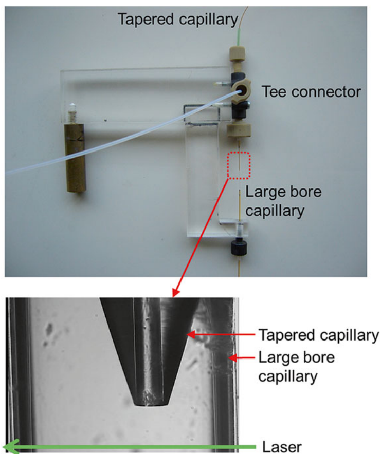
Fig. 1 Photos of the capillary holder ( upper ) and the tip of the tapered capillary inserted into the large bore capillary ( lower )
